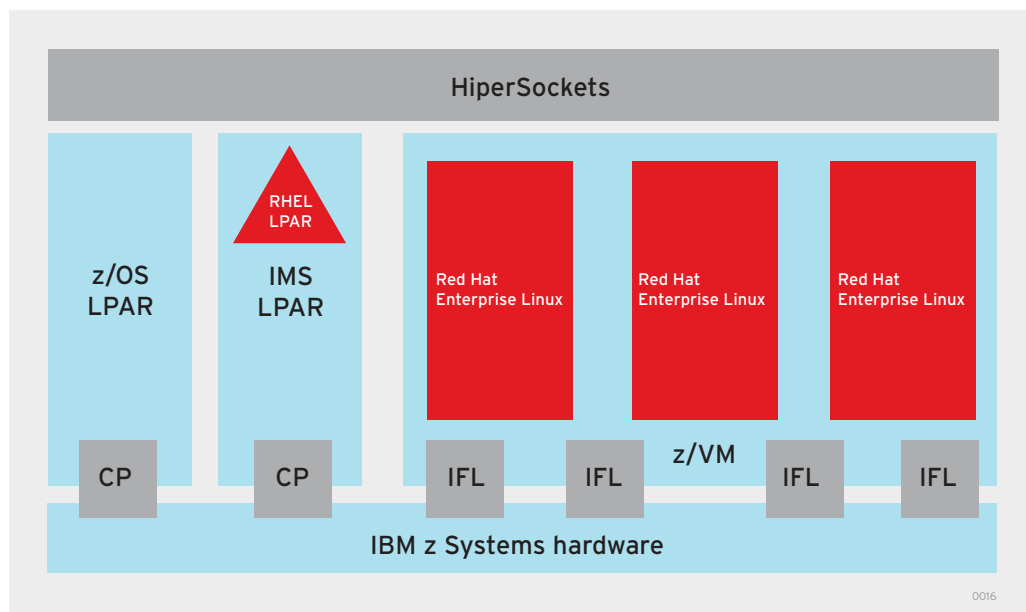
Figure 1. Red Hat Enterprise Linux on IBM z Systems Architecture
