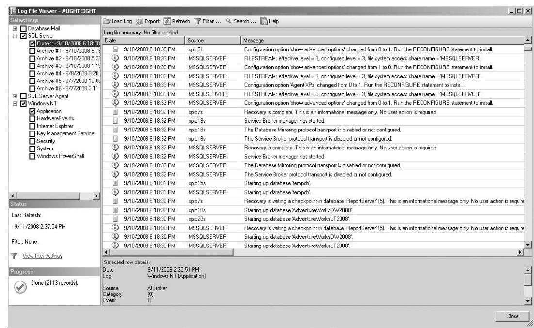
Figure 10-2: Log File Viewer.
