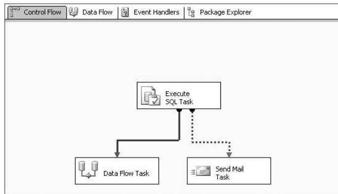
Figure 16-16: Control flow.
