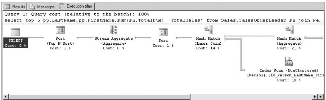
Figure 11-9: Execution plan after plan guide.
