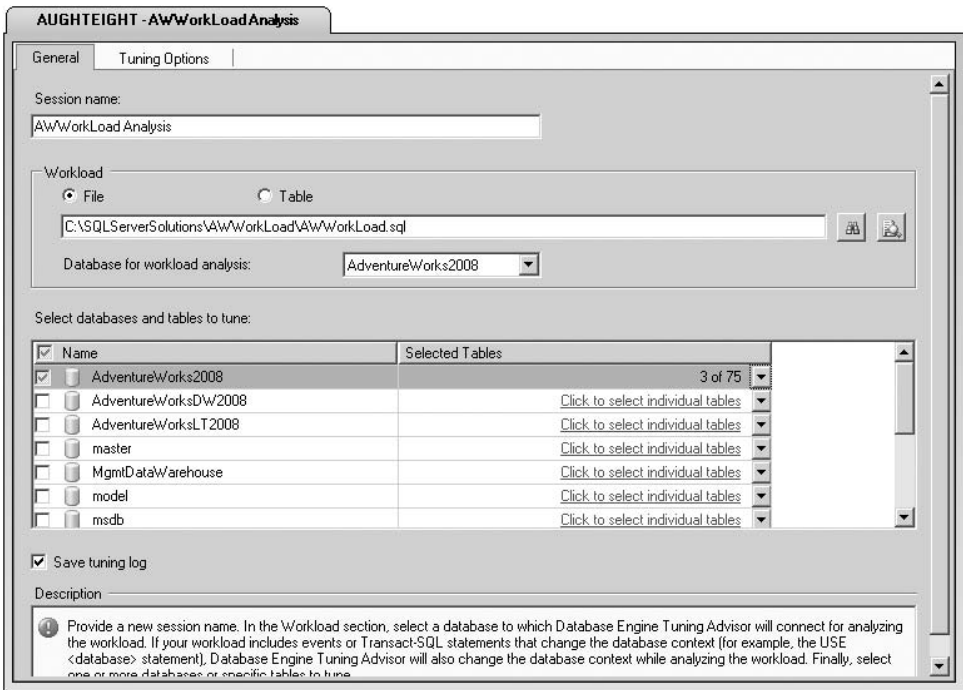
Figure 11-11: Starting a new session.
