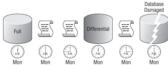
Figure 9-13: Full and Differential with Log scenario.
