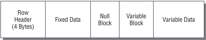
Figure 4-3: Header identifying a row.
