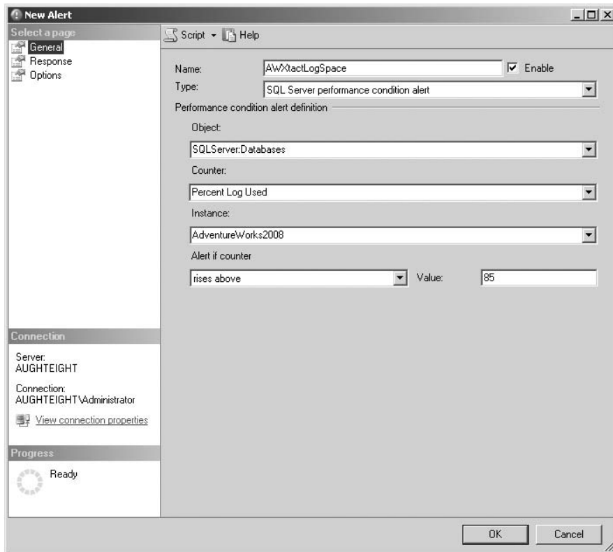
Figure 8-31: Creating a performance condition alert.
