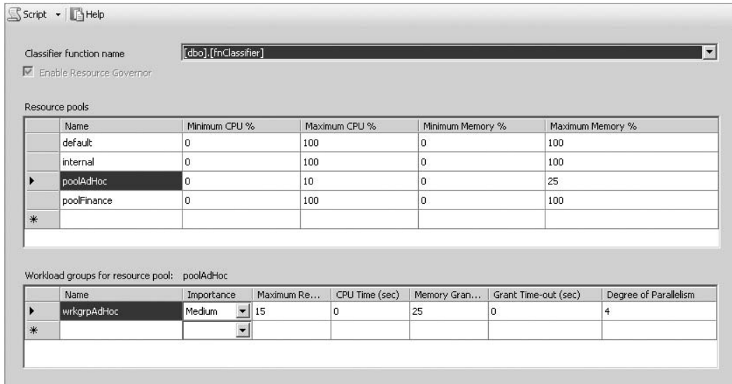
Figure 11-18: Resource Governor configuration.
