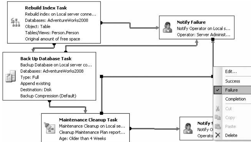
Figure 8-36: Maintenance Plan precedent constraints and tasks.
