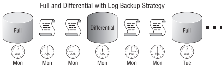
Figure 9-5: Full and Differential with Log backup strategy.
