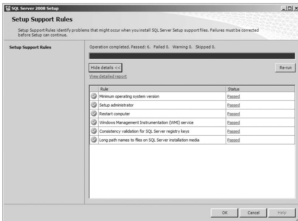
Figure 2-5: Setup Support Rules results for setup files.
