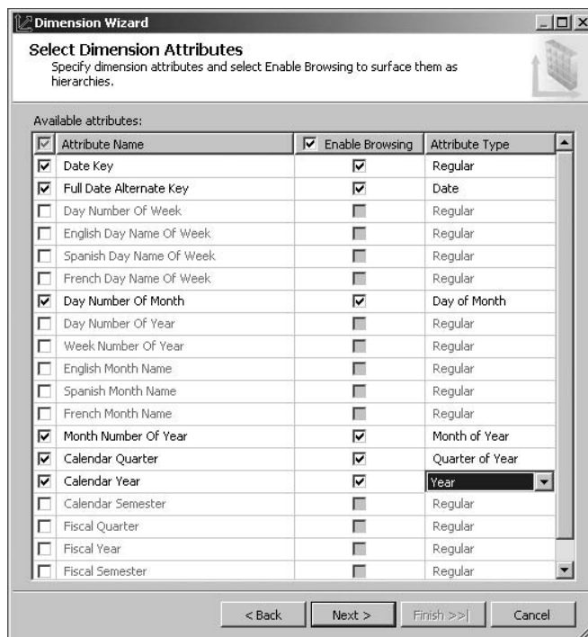
Figure 17-5: Enabling browsing on Date dimension attributes.
