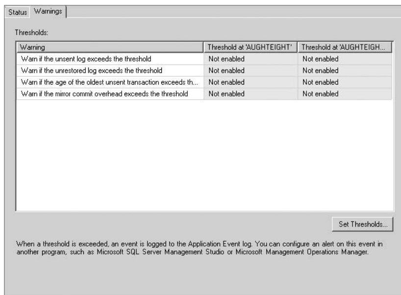
Figure 12-19: Configuring alert thresholds.
