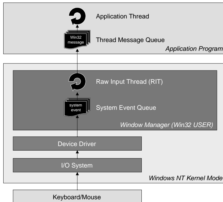
Figure 1: Windows NT Architectural Components for User Input
